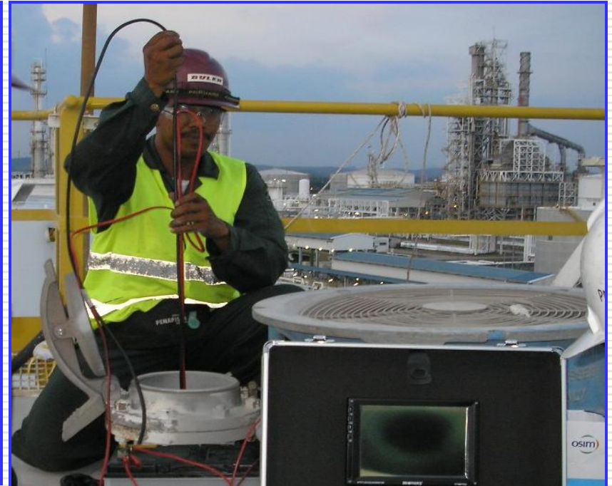
CCTV Inspection to Pipe Internal
