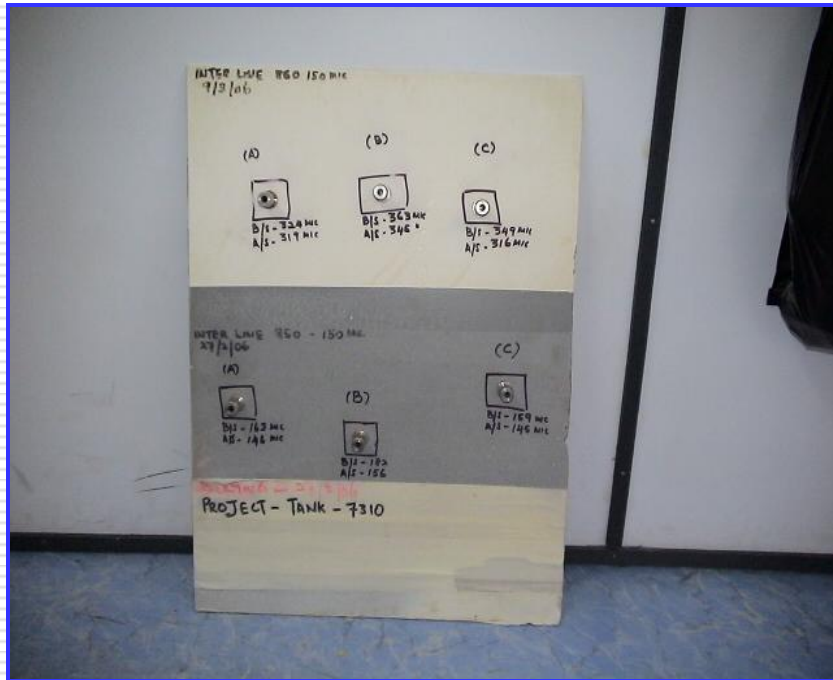
Test Plate Mounted with Dolly for Pull Off Test
