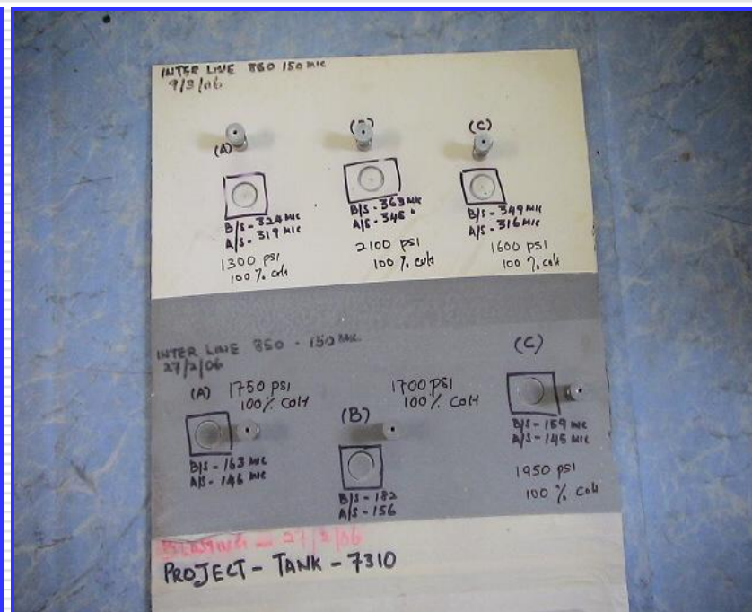
Successful Pull-Off Test Results – 2 nd Three Test
