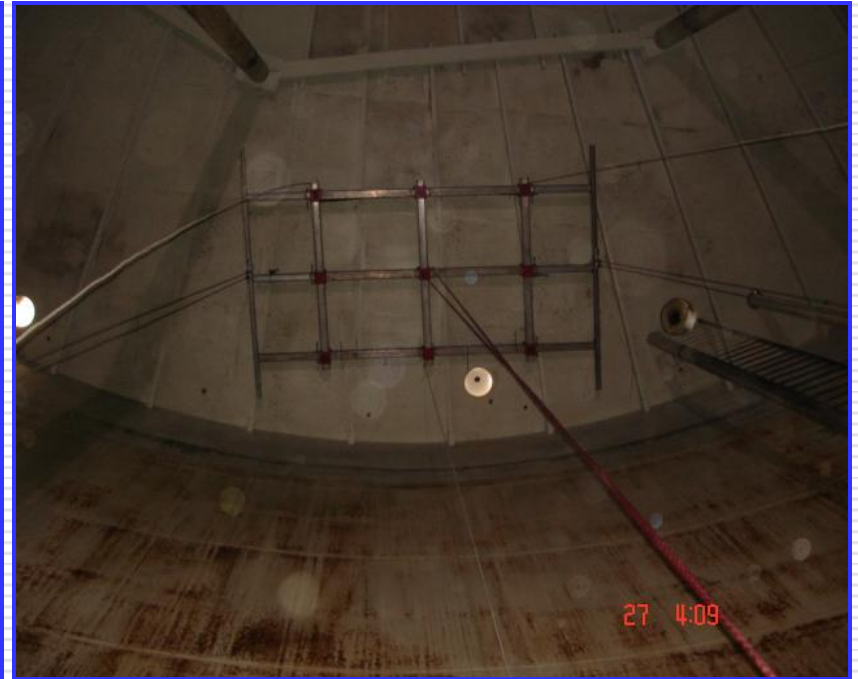
Securing of the Spreader System to Roof Underside
