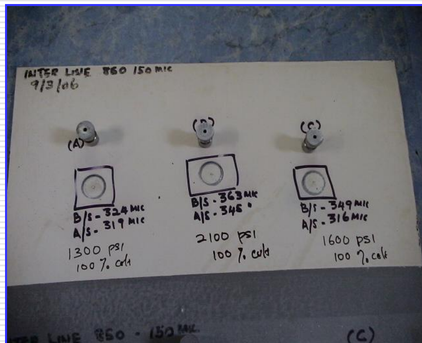
Successful Pull-Off Test Results – 1 st Three Test
